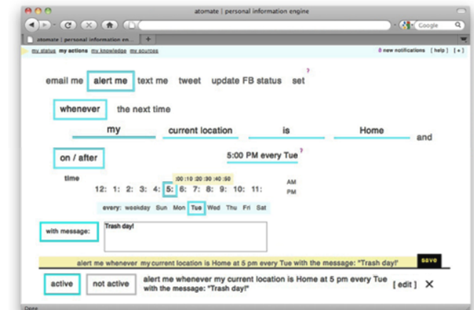
Figure 2: Top: A step-by-step montage illustrating the construction of the reminder behavior described in Scenario 1, using Atomate's constrained simplified natural language UI (CNLI). Bottom: The completed behavior.
